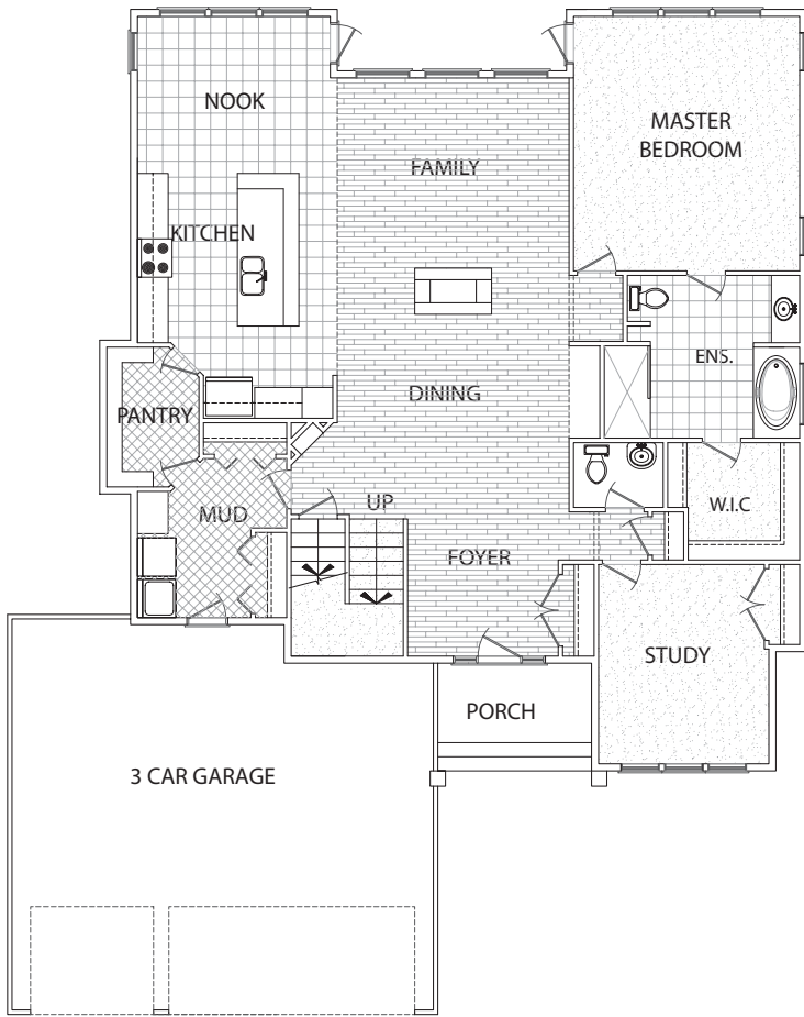
MAIN FLOOR PLAN 1887 sq. ft.
