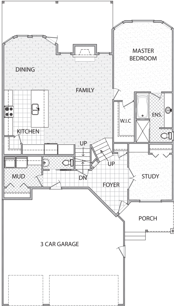
MAIN FLOOR PLAN 1567 sq. ft.
