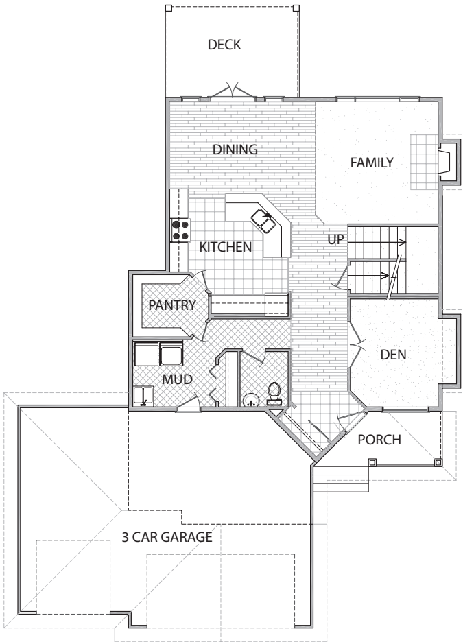
MAIN FLOOR PLAN 1138 sq. ft.
