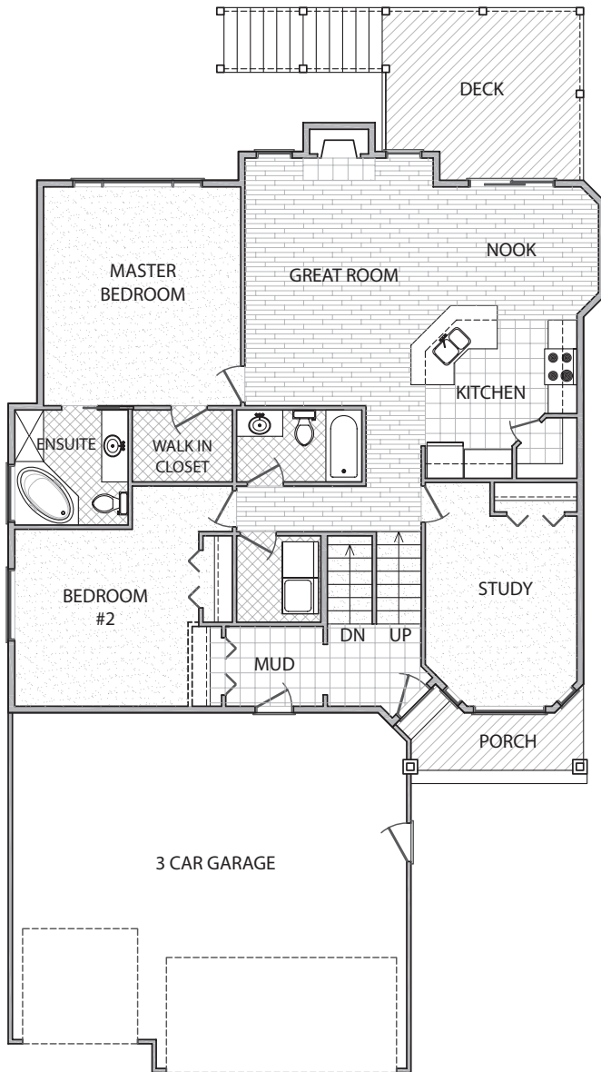
UPPER FLOOR PLAN 1482 sq. ft.
